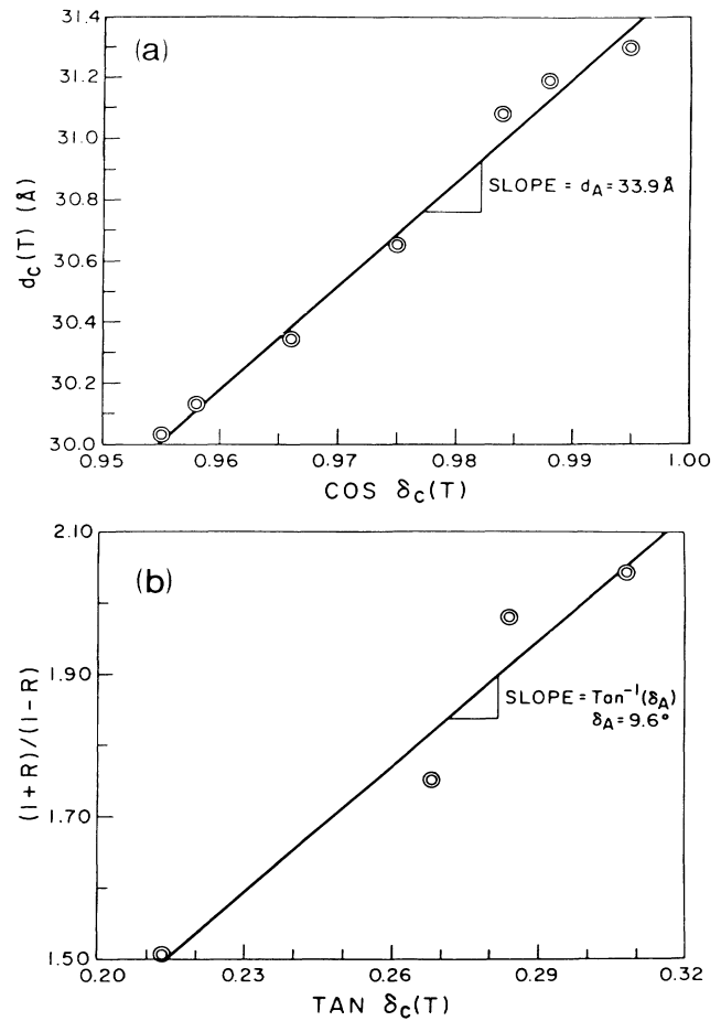
FIG. 4. (a) SmC layer spacing d_C(T) vs \cos\delta_C(T) , the SmC layer tilt angle. The slope is d_A = 33.9 \text{ \AA} which compares well with the 2\theta determined value of 31.4 \text{ \AA} . (b) (1 + R)/(1 - R) vs \tan\delta_C , where R = I_s/I_b is the intensity ratio of the two scattering peaks.
