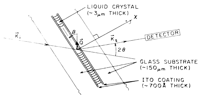
FIG. 1. The scattering geometry.
