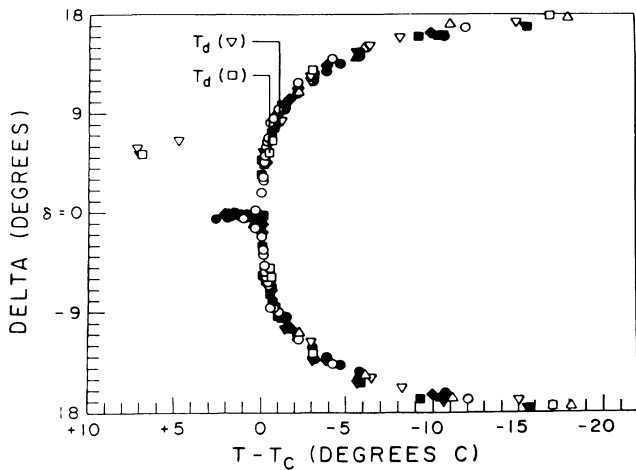
FIG. 3. Layer tilt \delta as a function of T - T_c , as obtained from the peak location in I(\beta) data, showing upper and lower branches located symmetrically about \delta = 0 . (Solid points, rotating anode; open points, SSRL.) The data yield no distinction among the various surface treatments used (see text). With the exception of the open inverted triangle and open square data, the points lie on a common curve with \delta \rightarrow 0 as T \rightarrow T_c and \delta_A = 0 in the SmA phase. For the open inverted triangles and open squares the SmA layers were tilted with \delta_A \approx 7^\circ in both the SmA and SmC phases for T > T_d = T_c - 1^\circ\text{C} , the temperature at which the peak on the lower branch appears with decreasing T . This and the fact that the open inverted triangle and open square data lie on the common curve for T < T_d indicate the formation of the asymmetric chevron for T < T_d .
