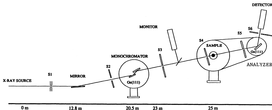
FIG. 1. The experimental layout at the NSLS beam line X10A. The x-ray beam was focused in the horizontal plane by an upstream bending mirror and then monochromated by a double-bounce Ge(111) crystal. The analyzer was a single-bounce Ge(111) crystal. The out-of-plane resolution was achieved by three sets of slits (S1, S3, S5). S1 and S3 define the spot size at the sample position. S2, S4, and S6 are primarily used to cut out stray air scattering.
