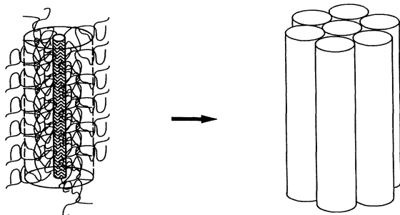
FIG. 4. A schematic representation of the formation of two-dimensional lattices of the close-packed tubular aggregates. The tubelike aggregate has a polar core region where the zwitterionic heads reside surrounded by the polyisoprene tails which are relatively stretched out.
