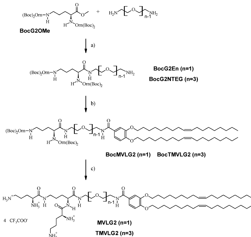
Figure 3. Synthesis of the dendritic cationic lipids MVLG2 ( n=1 ) and TMVLG2 ( n=3 ); \text{Orn}(\text{Boc})_2 = \text{C}(\text{O})\text{CH}(\text{NHBoc})(\text{CH}_2)_3\text{NHBoc} . Reaction conditions: (a) excess diamine (20 \times ) in MeOH; (b) DOB, TBTU, HOBt, DIEA; (c) TFA. DOB: 3,4-dioleoyloxybenzoic acid; HOBt: 1-hydroxybenzotriazole hydrate; DIEA: N,N -diisopropylethylamine; TBTU: O -benzotriazol-1-yl- N,N,N',N' -tetramethyluronium tetrafluoroborate; TFA: trifluoroacetic acid.
