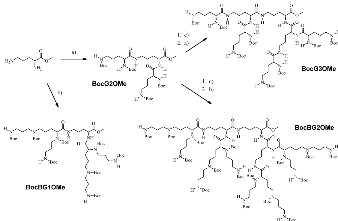
Figure 2. Synthesis of the dendritic headgroup building blocks, starting from ornithine methyl ester. Reaction conditions: (a) Boc-ornithine, TBTU, HOBt, DIEA; (b) Boc-carboxyspermine, TBTU, HOBt, DIEA; (c) TFA. HOBt: 1-hydroxybenzotriazole hydrate; DIEA: N,N -diisopropylethylamine; TBTU: O -benzotriazol-1-yl- N,N,N',N' -tetramethyluronium tetrafluoroborate; TFA: trifluoroacetic acid.
